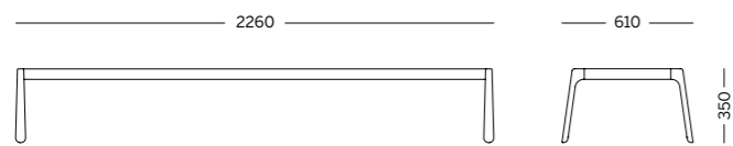
MODULE D - Structure for 4 units
