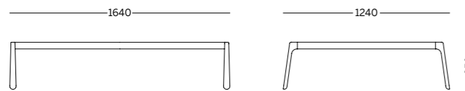
MODULE E - Double structure for 3 units per side
