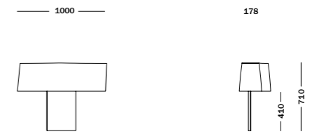
MODULE R - Left curved backrest
